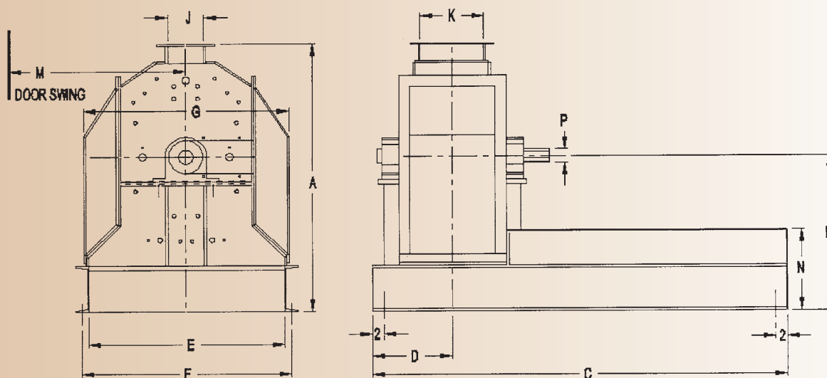
MILL DIMENSIONS (INCHES)
